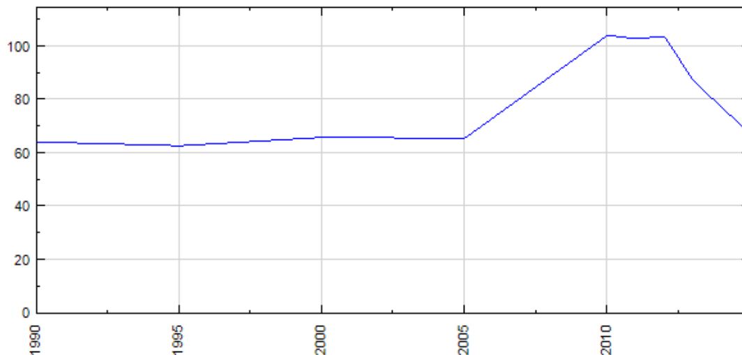
FIGURE 17: PM2.5 AIR POLLUTION, MEAN ANNUAL EXPOSURE ( \mu\text{m}^3 ) 15
